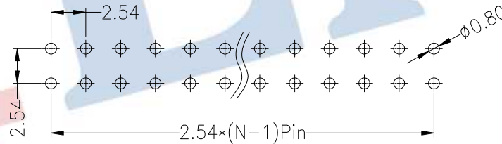
Recommended P.C.B Layout(Top Side) (PCB BOARD TOLERANCE±0.05)
